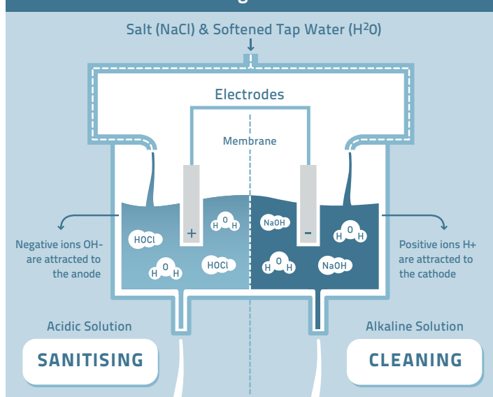
Cross section diagram of ROX10® unit
